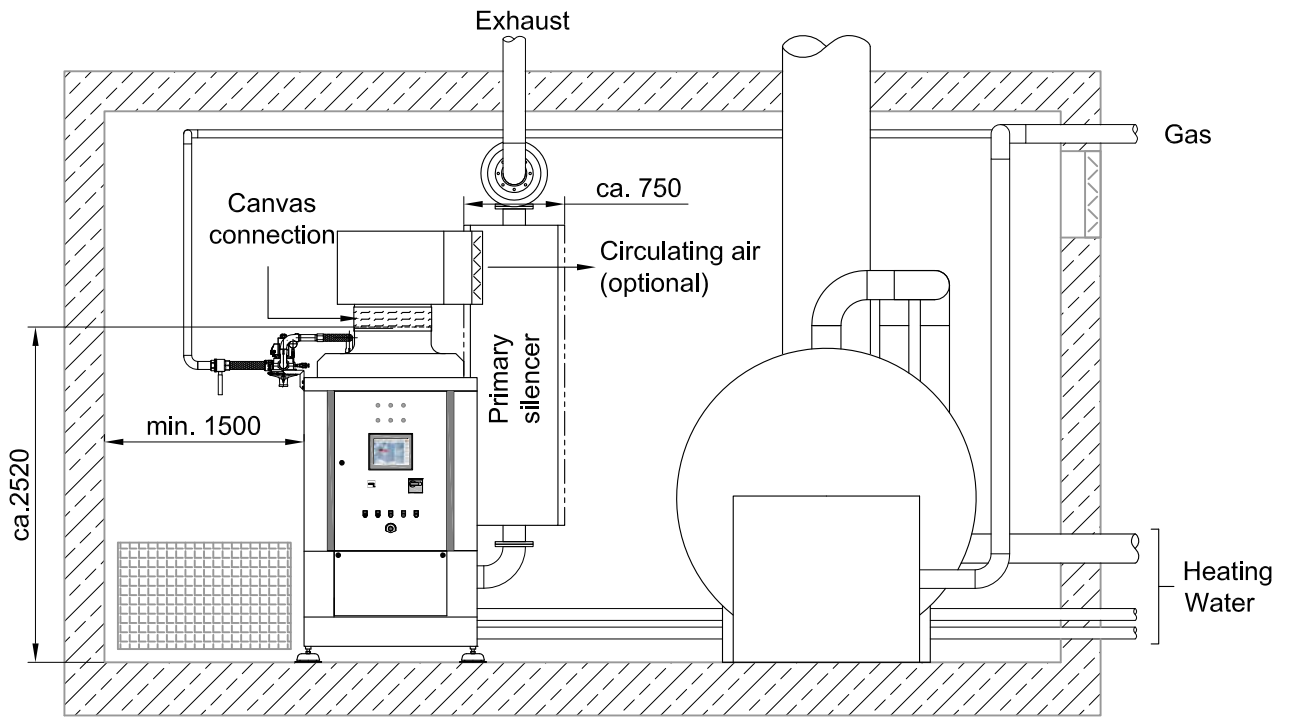
Sectional view
